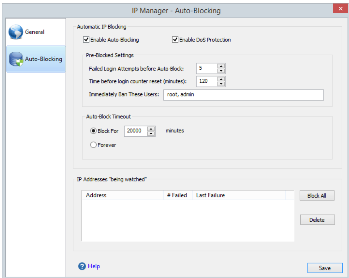
Figure 34 Auto-blocking page of the IP Manager
