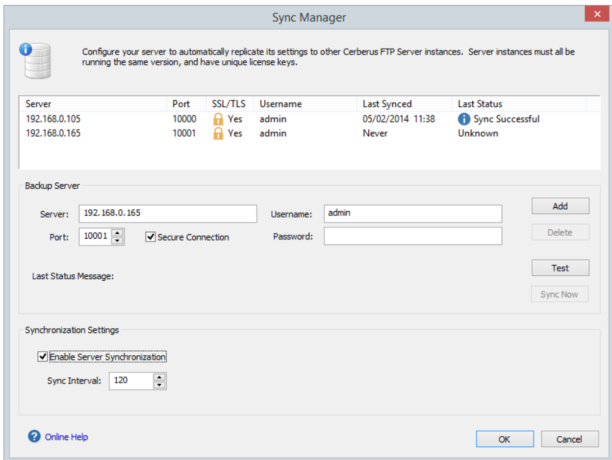
Figure 47 Cerberus Synchronization Manager
