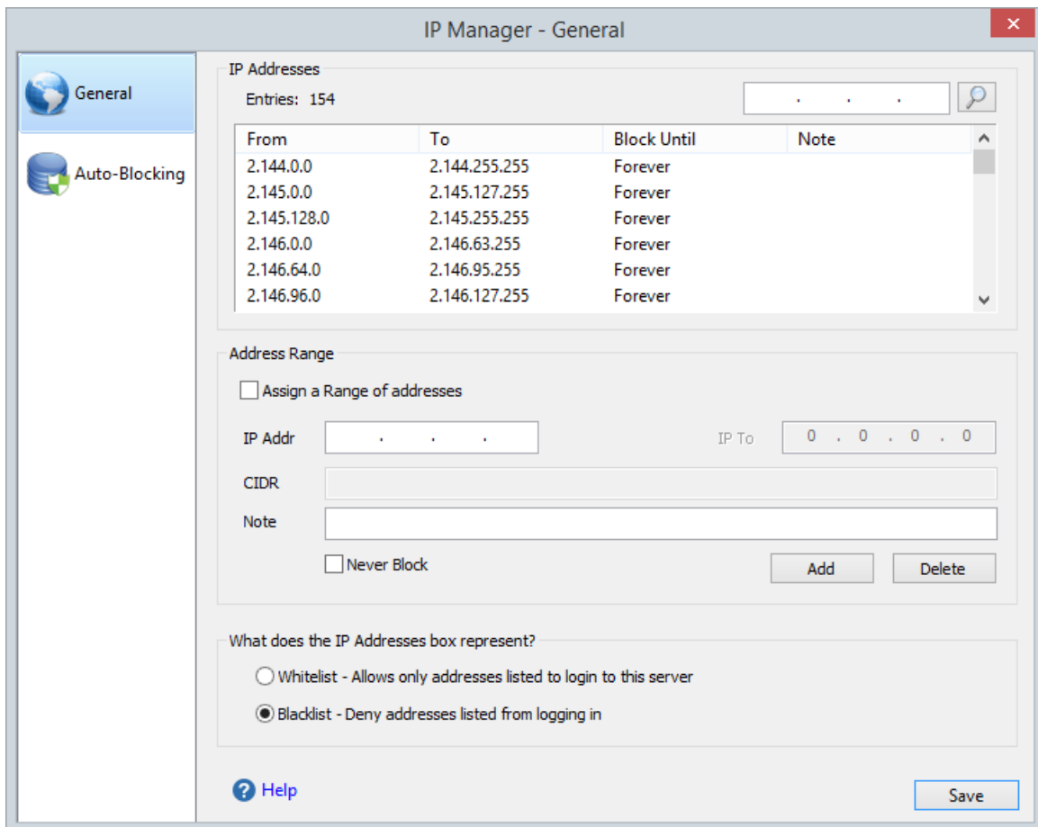
Figure 33 General page of the IP Manager
