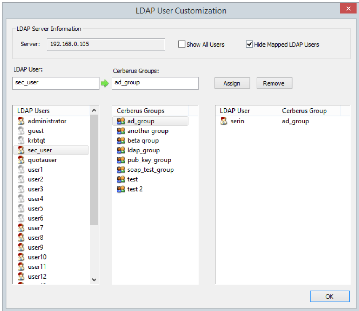
Figure 43 Configuration page for LDAP User to Cerberus Group Mapping
