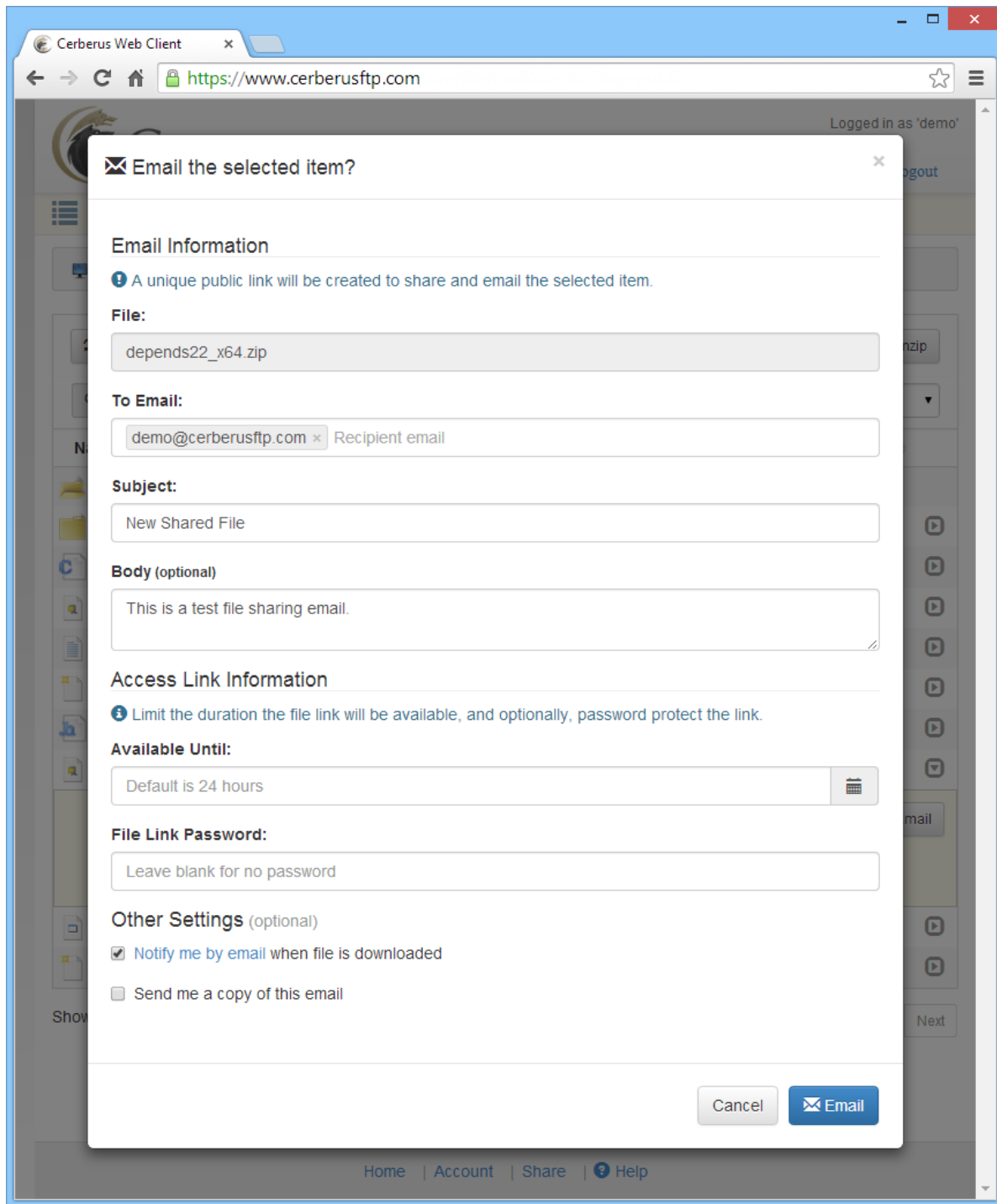
Figure 21 Cerberus FTP Server HTTP/S Web Client
