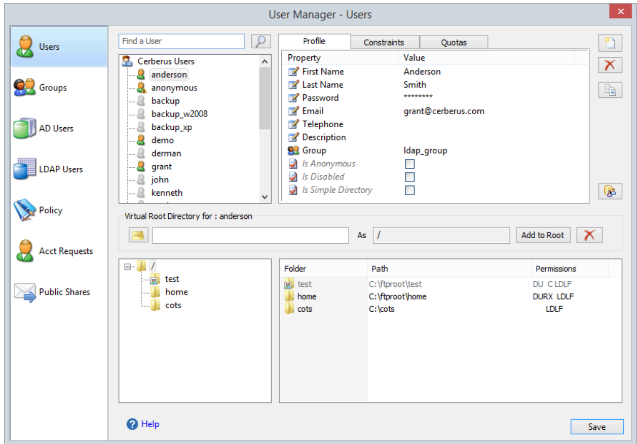
Figure 7 - The Cerberus FTP Server User Manager- Users page
