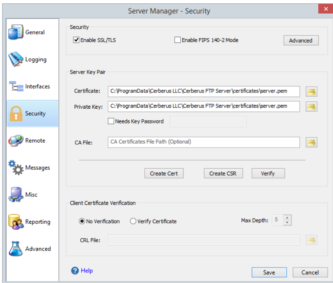
Figure 50 Security settings page of the Server Manager
