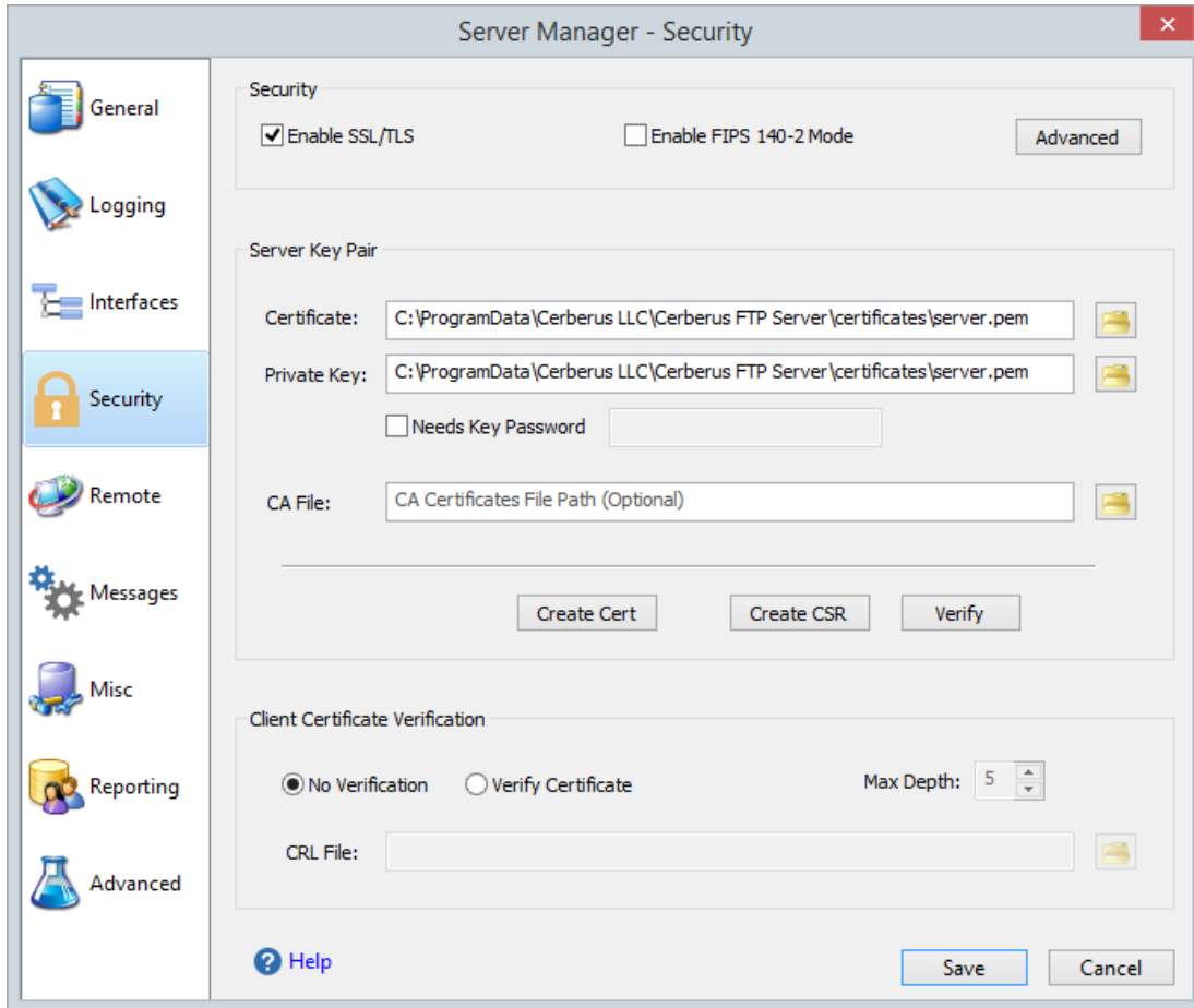
Figure 27 Security settings page of the Server Manager
