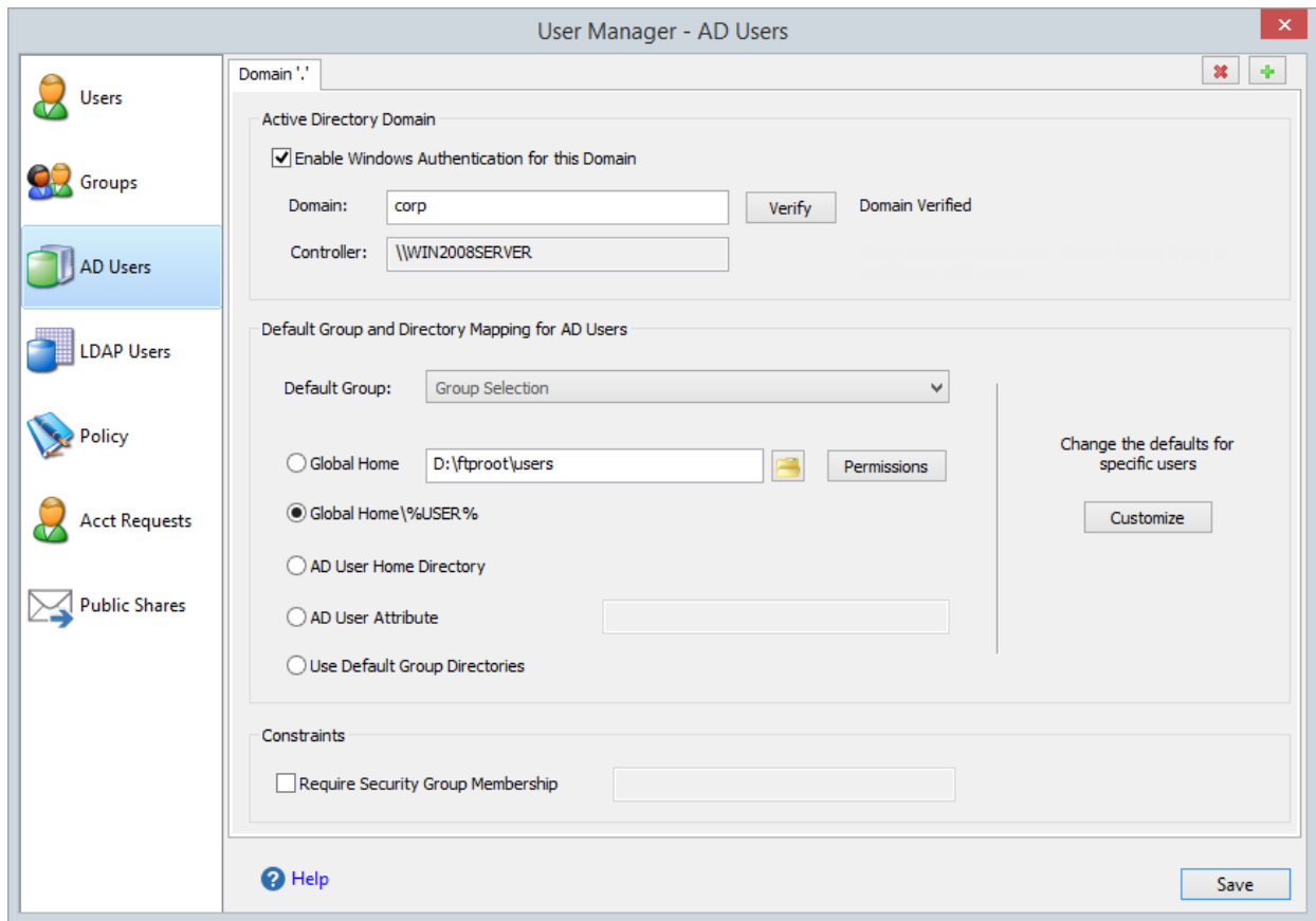
Figure 44 Active Directory Authentication page
