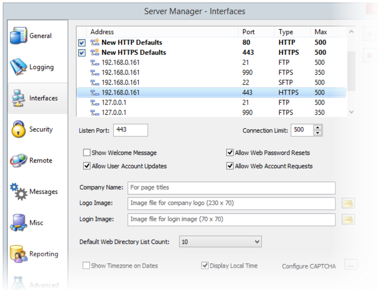
Figure 22 Cerberus FTP Server HTTP Listener
