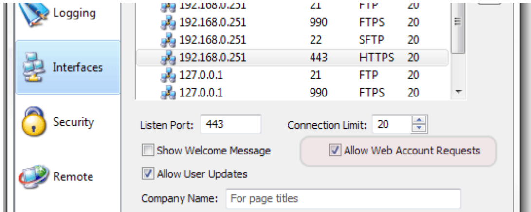
Figure 25 Enabling or disabling allowing Account Requests
