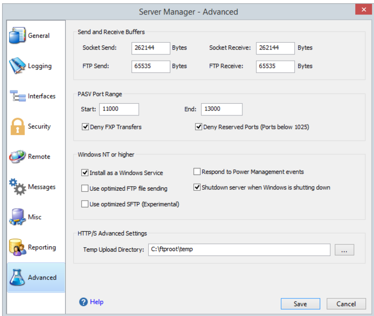
Figure 32 Advanced page of the Server Manager
