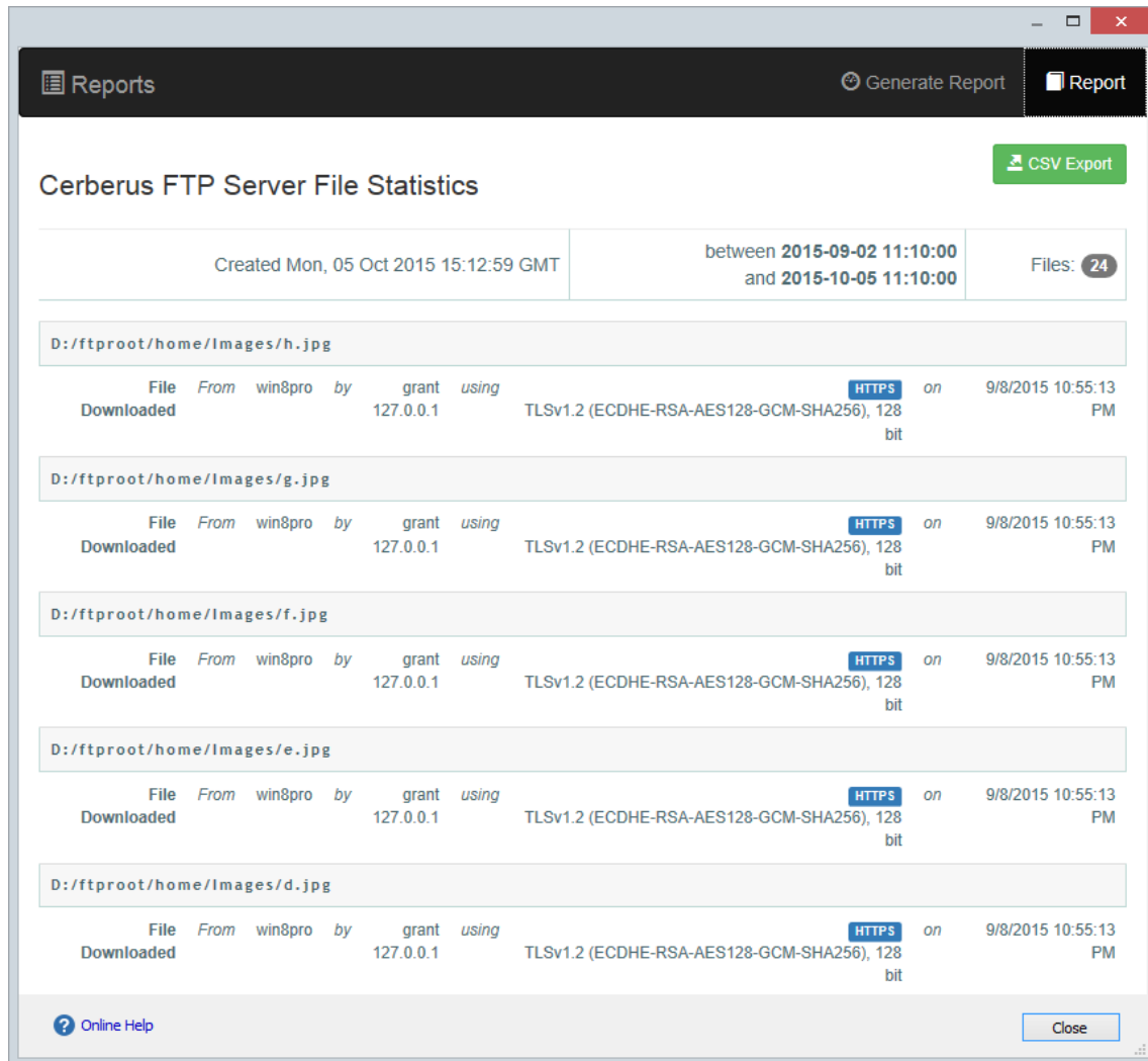
Figure 41 Cerberus FTP Server File Access Report, Filtered by Date
