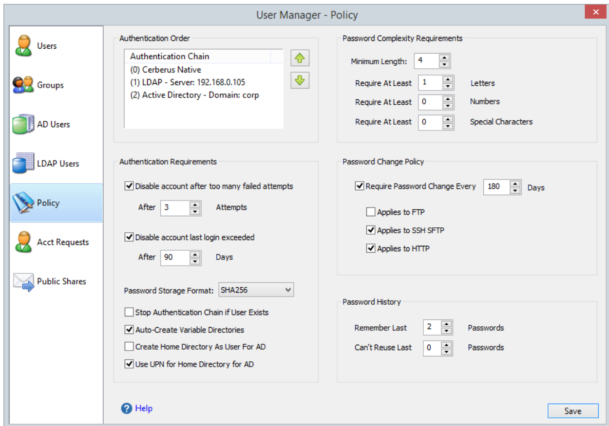
Figure 13 User Manager Policy Page
