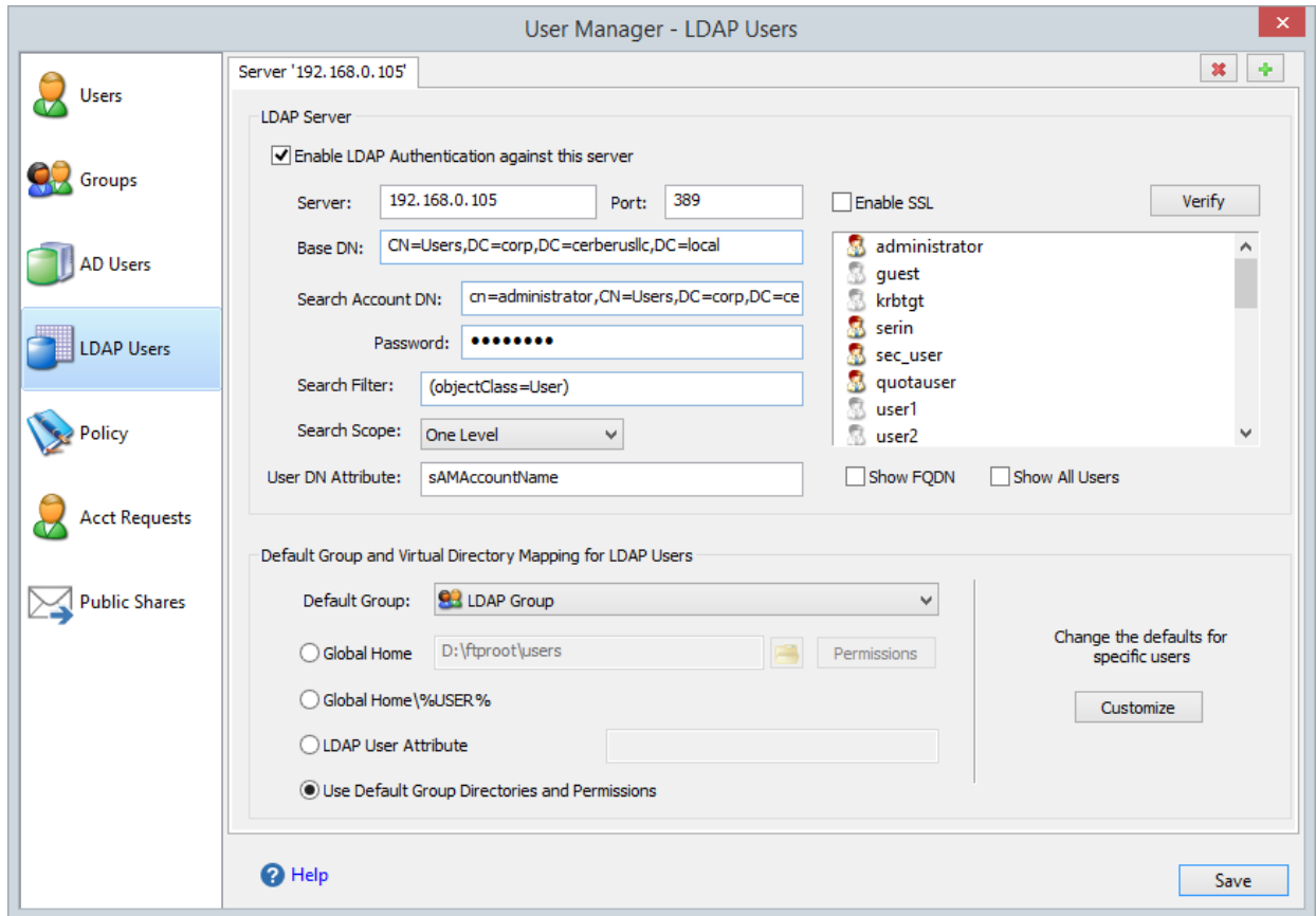
Figure 42 Configuration page for LDAP Authentication
