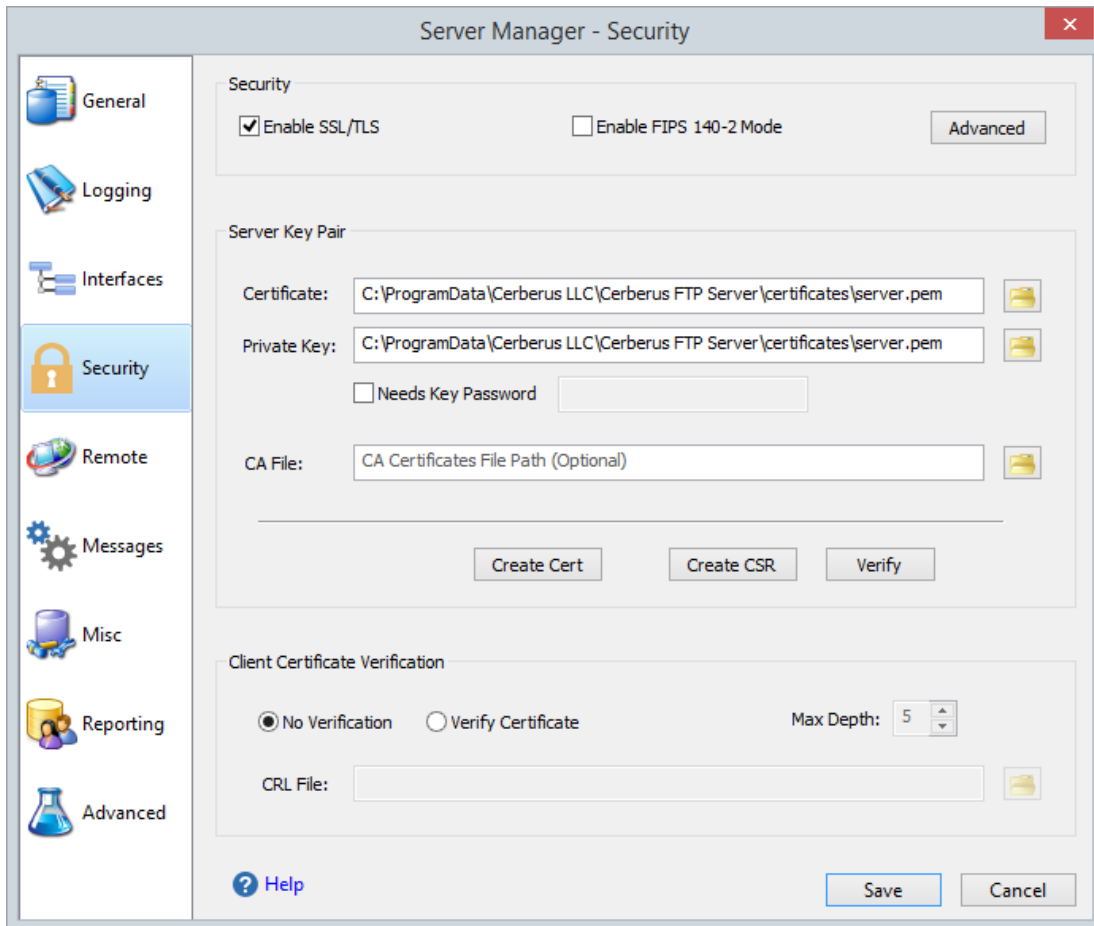
Figure 49 Security settings page of the Server Manager
