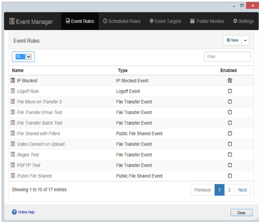
Figure 36 Rules List page of the Event Manager
