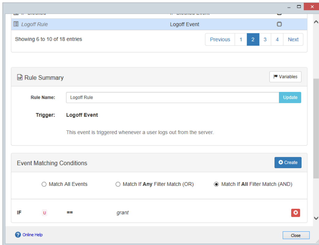
Figure 37 Rule Editing in the Event Manager
